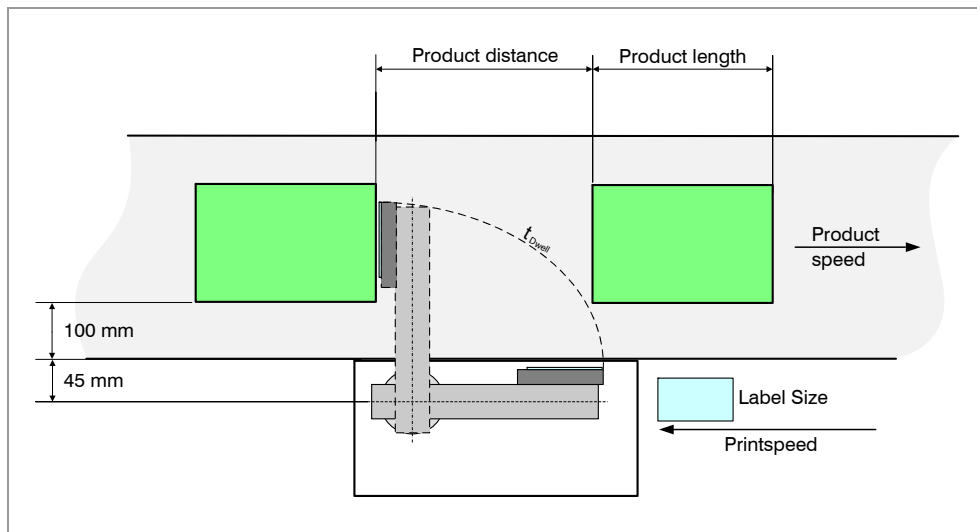
[5] LA-SO example application (schematic).
