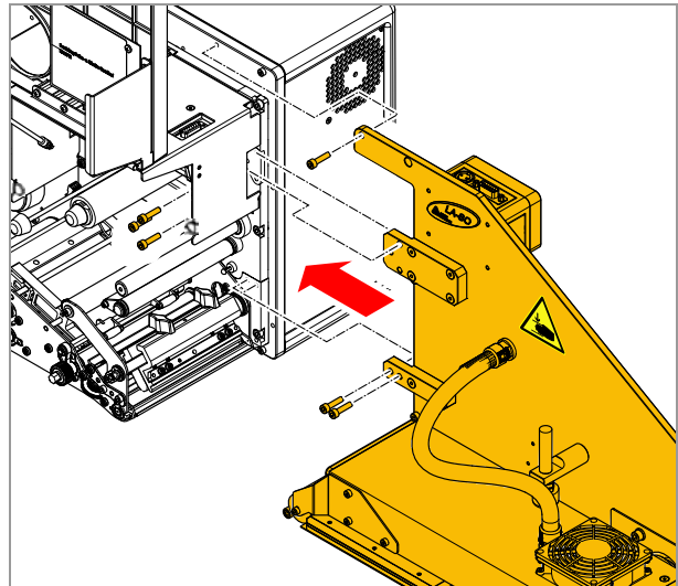
[14] Mounting the LA-SO on an ALX 92x.
