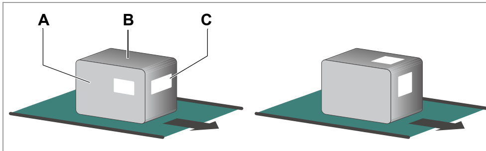
[7] Designations for the sides of the product. Possible label positions for side labelling (left figure) and top labelling (right figure).
