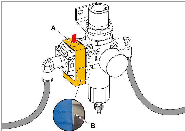
[21] Slide of the on-off valve in „open“ position (B).
