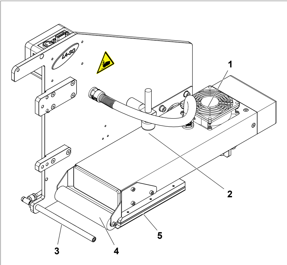
[11] LA-SO (RH), front.
