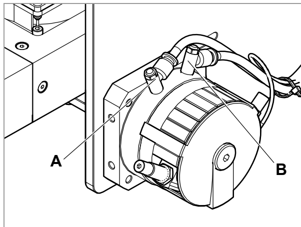
[20] Swivel module of LA-SO (RH).
