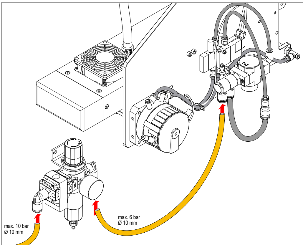
[19] Connecting the compressed air hose.
