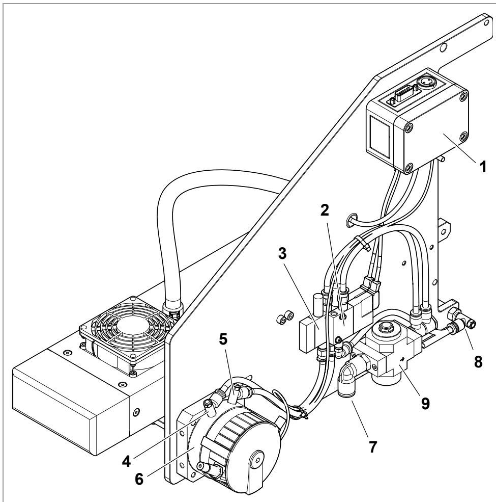
[12] LA-SO (RH), rear.
