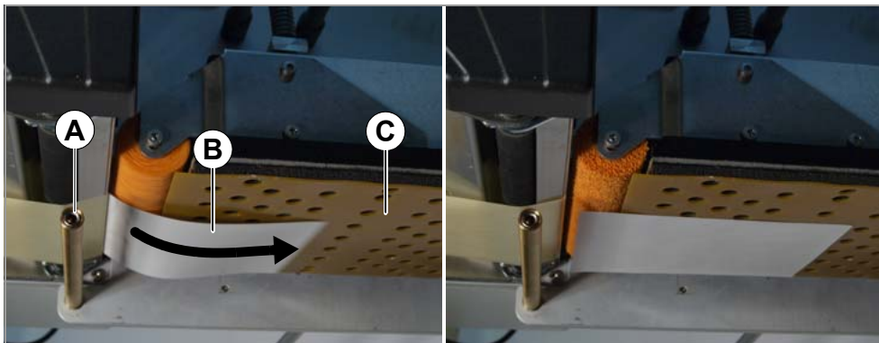
[8] Dispensing labels onto the pressure plate.
