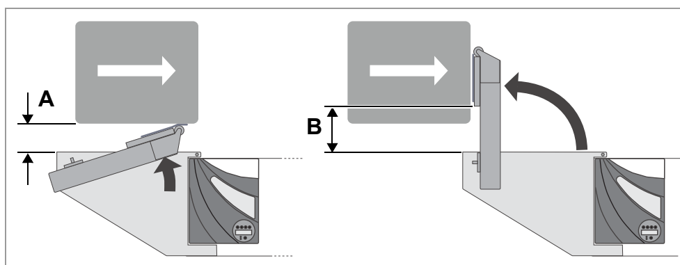
[6] Application distance. Left: label on side. Right: label on front.
